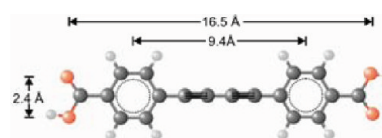
Figure 1. Chemical structure of the 4,4'-di-(1,4-buta-1,3-diynyl)-benzoic acid with carboxylic and alkyne functionalities (H, white; C, gray; O, red).
