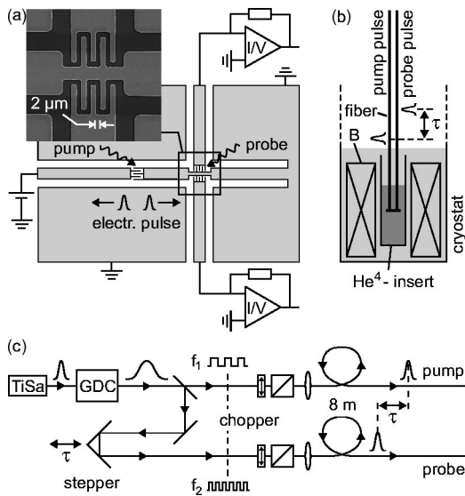
FIG. 1. (a) Schematic diagram of the coplanar waveguide circuit. The inset shows a scanning electron microscopy picture of the twin probe-switch. (b) Sketch of a fiber coupled sample in the ^4\text{He} bath-cryostat. (c) Optical setup for the PC sampling experiments.
