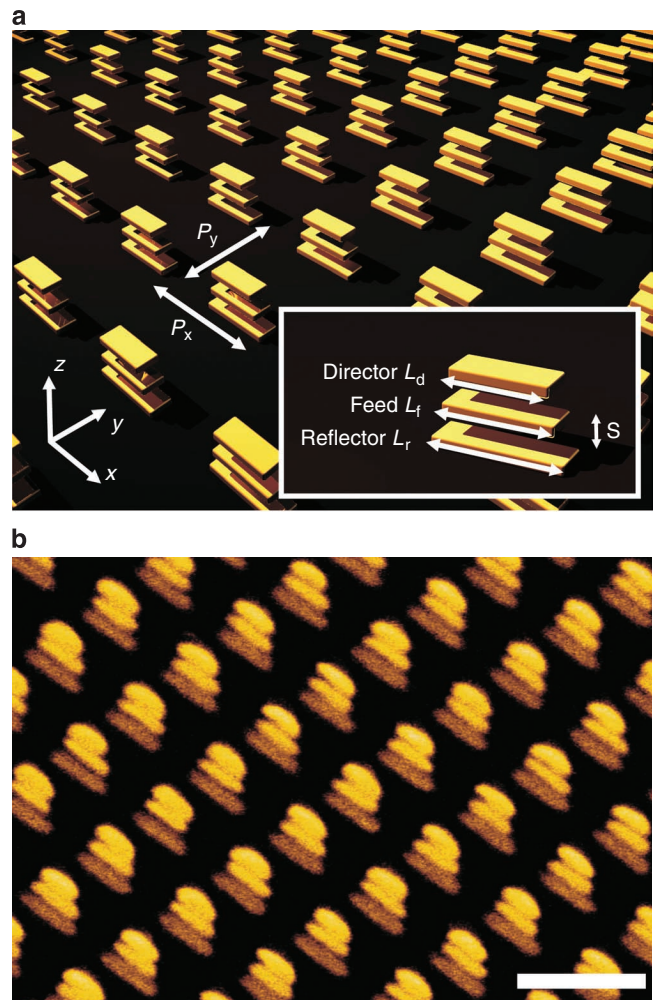
Figure 1 | The optical Yagi–Uda antenna array. (a) Schematic picture of the optical Yagi–Uda antenna array. The period in x -direction is P_x = 450 nm and in y -direction P_y = 300 nm. The inset shows the single antenna with definitions of the geometrical parameters: L_r = 300 nm, L_f = 250 nm, L_d = 230 nm and S = 100 nm. (b) Scanning electron microscope image of the optical Yagi–Uda antenna array. The gold structure is fabricated on a glass substrate. The nanorods are embedded in a photopolymer (PC403), which serves as the dielectric spacer. Scale bar, 500 nm.
