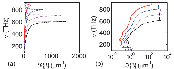
FIG. 2. (Color online) (a) Real and (b) imaginary part of the propagation constant \beta of the lowest order PSPP mode as a function of frequency \nu for selected values of \epsilon_d : \epsilon_d = 1 (solid red), \epsilon_d = 2.8 (dashed blue), \epsilon_d = 5.4 (dotted magenta), \epsilon_d = 9 (dotted-dashed black). The inset shows the H_\phi -field norm for a core radius of 10 nm and \epsilon_d = 1 .
