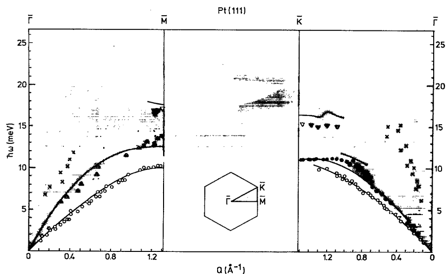
FIG. 3. Measured and calculated dispersion curves for Pt(111) (see text). Only theoretical dispersion curves with a vertical component are shown.
