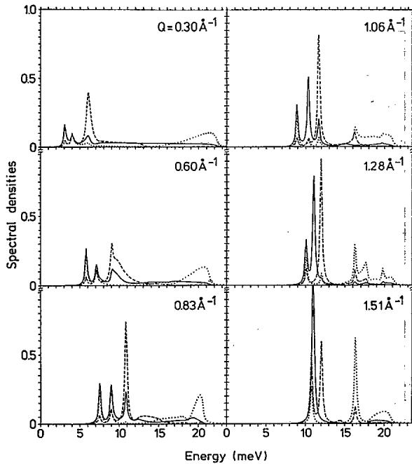
FIG. 5. Phonon spectral density series of Pt(111) along the \bar{\Gamma} - \bar{K} azimuth with Q as a parameter. The notation and constants are the same as in Fig. 4 ( Q = 1.51 \text{ \AA}^{-1} at the \bar{K} point).
