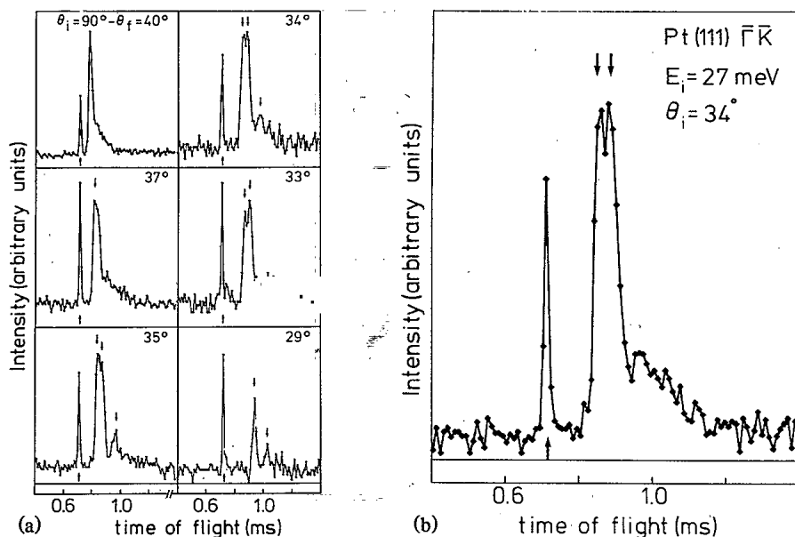
FIG. 1. (a) Series of TOF spectra for the \bar{\Gamma} - \bar{K} azimuth at a crystal temperature of 25 K and a He-beam energy of 27 meV. With decreasing incident angle \theta_i , phonons with higher phonon momentum and energy are probed. (b) TOF spectrum at \theta_i=34^\circ with improved signal to noise ratio, 3.5 h measuring time.
