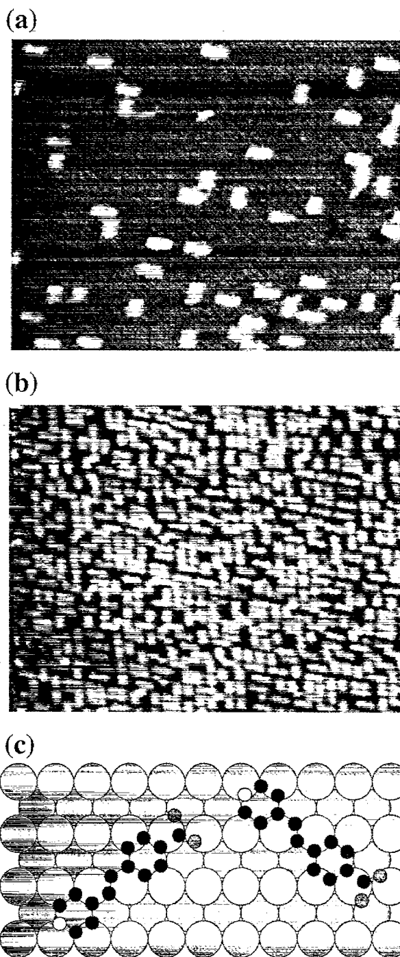
Fig. 4. STM images of PVBA molecules on Pd(110) with (a) submonolayer coverage ( T = 360 K) and (b) monolayer coverage ( T = 410 K); image sizes: 210 \times 170 \text{ \AA} (c) ball model of the adsorption geometry. The PVBA molecules may be shifted by half an atom along the Pd rows.
