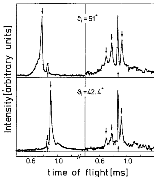
FIG. 2. He TOF plots taken in the \bar{\Gamma}\bar{M} direction from the clean (left) and the p(2 \times 2) O/Pt(111) surface (right). E_{\text{He}} = 17.4 \text{ meV} , T_s = 300 \text{ K} . The diffuse elastic peaks are denoted by arrows pointing up.
