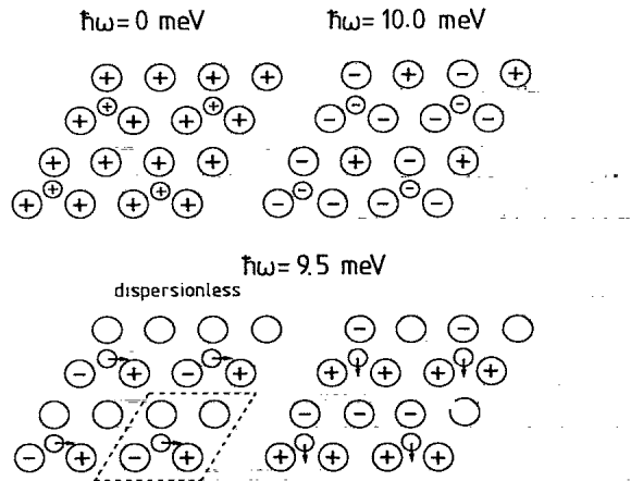
FIG. 4. Sketch of the four eigenmodes of the p(2 \times 2)O/Pt(111) surface as they result from the dynamical analysis at the \bar{\Gamma} point.
