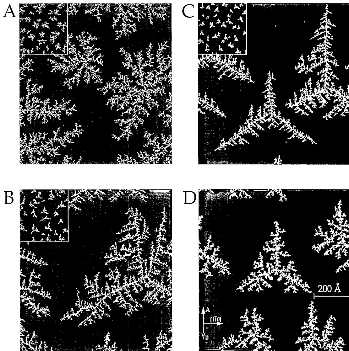
Fig. 4. KMC simulations of the STM experiments for Ag/Pt(111). As in Fig. 1A, the scale is the same for figures and insets, they correspond to growth temperatures of 130 and 80 K, respectively. Coverages and deposition rates are as in the experiment. For hit and stick, classical DLA fractals result (A). The key process for dendritic islands is diffusion from corner to A-steps (B). Close-packed chains that occasionally form in (B) are no more observed when a small atomic row is allowed to relax (C). Best agreement with experiment is obtained when corner to B-step diffusion is introduced (D).
