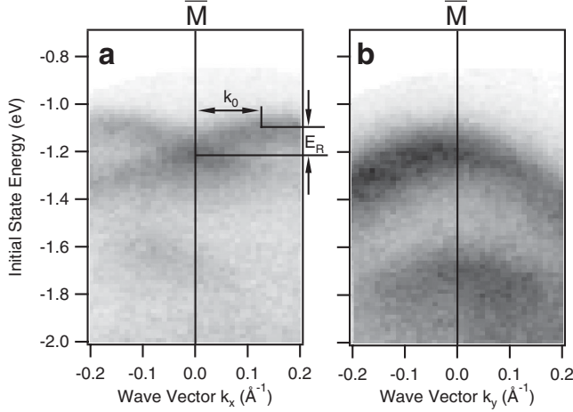
FIG. 3. Experimental band structure of Bi/Si(111) near the \bar{M} -point. The measurements along \bar{\Gamma} \bar{M} \bar{\Gamma} (a) and \bar{K} \bar{M} \bar{K} (b) show the anisotropic topology of the spin-split bands.
