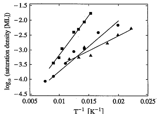
FIG. 2. Arrhenius plot of saturation island densities derived from STM for nucleation of Ag on Pt(111) (■), on 1 ML Ag adsorbed on Pt(111) (▲), and on Ag(111) (●), respectively.
