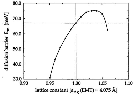
FIG. 3. Barrier for Ag self-diffusion on a Ag(111) slab as a function of tensile or compressive strain as calculated with EMT.
