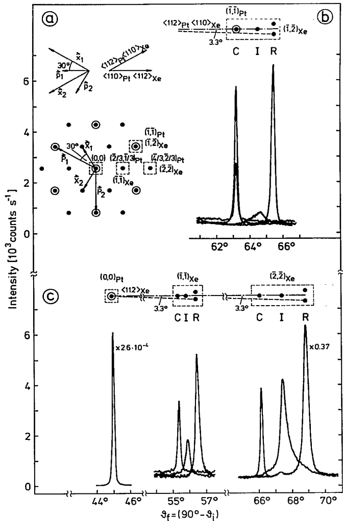
FIG. 1. Polar scans of He diffraction from clean and Xe-covered Pt(111). (a) Real- and reciprocal-space representations; p_i and x_i are the real-space and P_i and X_i the reciprocal-space basis vectors of the Pt(111) surface and of the commensurate (\sqrt{3} \times \sqrt{3})R30^\circ Xe lattice, respectively; the indexed dashed squares mark the diffraction peaks plotted. (b) Polar scan of the (\bar{1}, \bar{1})_{Pt} and of the (\bar{1}, \bar{2})_{Xe} commensurate (C), incommensurate (I), and incommensurate-rotated (R) peaks. (c) Polar scan of the (0, 0)_{Pt} and of the (\bar{1}, \bar{1})_{Xe} and (\bar{2}, \bar{2})_{Xe} C, I, and R peaks.
