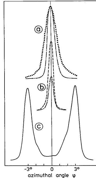
FIG. 2. Azimuthal profiles of He diffraction peaks from clean and Xe-covered Pt(111): (a) (\bar{1}, \bar{1})_{Xe} I (dotted) and C (dash-dotted); (b) (\bar{1}, \bar{1})_{Pt} (dashed) and (\bar{1}, \bar{2})_{Xe} C (dash-dotted); (c) (\bar{2}, \bar{2})_{Xe} R (solid). All peaks are normalized to the same height except for (\bar{1}, \bar{2})_{Xe} C which has the real relative height with respect to (\bar{1}, \bar{1})_{Pt} .
