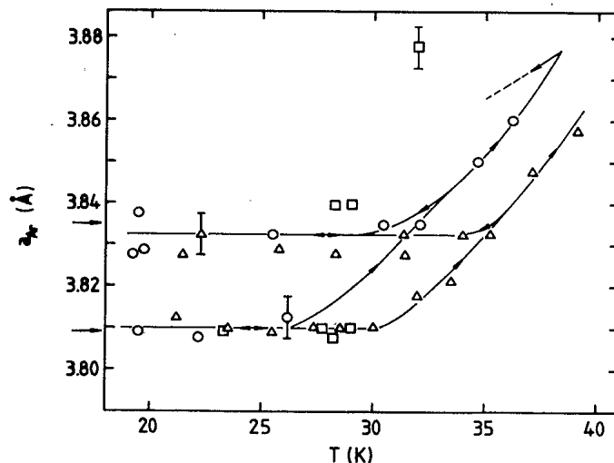
FIG. 7. Thermal expansion of the Ar adlayer in the low-coverage regime ( \Theta \approx 0.36 ML). The lines through the data demonstrate the irreversibility of the expansion. Different symbols correspond to different measuring runs. The two lattice parameter values marked by the arrows correspond to the theoretical Ar interatomic distance in the (11 \times 11)R0^\circ ( a_{Ar} = 3.809 Å) and the (18 \times 18)R0^\circ ( a_{Ar} = 3.835 Å) high-order commensurate phase, see Table I.
