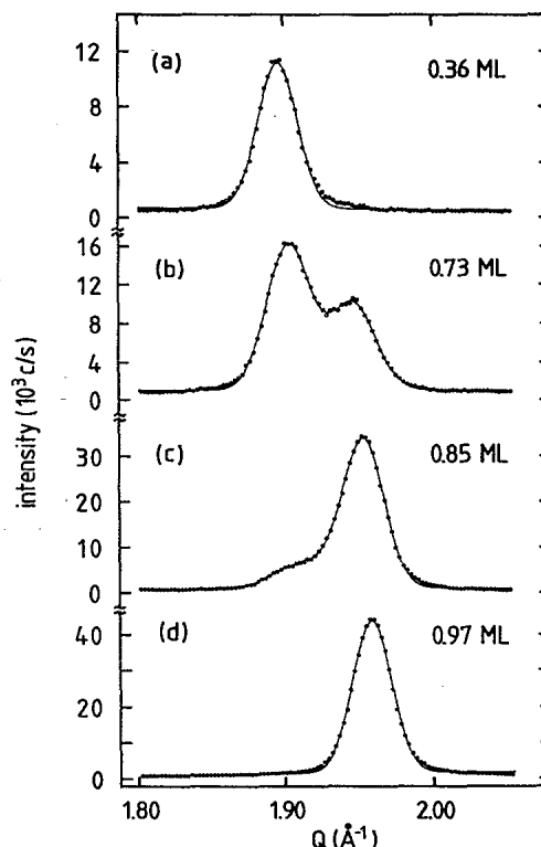
FIG. 3. Polar profiles of the (10)_{\text{Ar}} diffraction peak for different Ar coverages. Other experimental parameters as in Fig. 2. The solid lines through the data are best fits using Gaussian line shapes.
