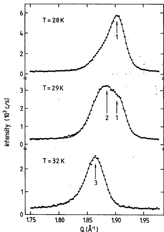
FIG. 8. Polar He diffraction profiles of the (10)_{\text{Ar}} peak in the low-Ar-coverage regime ( \Theta=0.36 \text{ ML} ) at different surface temperatures. The sequence (a)–(c) demonstrates the discontinuous transition between different Ar phases locked to the Pt(111) substrate: (1) a_{\text{Ar}}=3.81 \text{ \AA} ( Q=1.905 \text{ \AA}^{-1} ), (2) a_{\text{Ar}}=3.84 \text{ \AA} ( Q=1.890 \text{ \AA}^{-1} ), and (3) a_{\text{Ar}}=3.88 \text{ \AA} ( Q=1.870 \text{ \AA}^{-1} ). These spectra were recorded with a He beam energy of 17.5 meV. The solid lines are again best-fit Gaussians.
