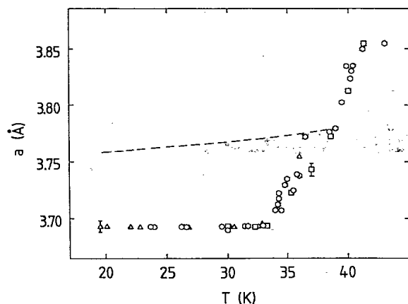
FIG. 4. Lattice parameter of the Ar monolayer as a function of surface temperature. Different symbols correspond to Ar adlayers with different total coverage in the range 0.85 \leq \Theta \leq 1 ML. The dashed line indicates the thermal variation of the interatomic distance in bulk argon (Ref. 18). This should be very close to the thermal expansion of an incommensurate overlayer as shown in the case of Kr/Pt(111) (Ref. 10).
