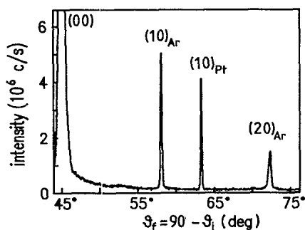
FIG. 2. Polar He diffraction profile along the \bar{\Gamma}\bar{M}_{\text{Pt}} azimuth from a 0.3-ML Ar adlayer physisorbed on Pt(111). He beam energy 18.3 meV, surface temperature T=25 K.
